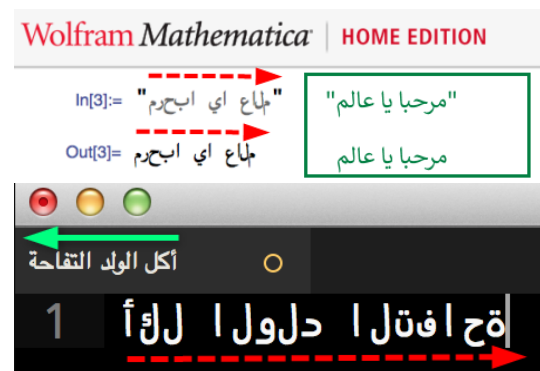
Figure 4. Right to left support when typing Arabic. Top (Mathematica): direction flipped for both sentence and words, and letters disconnected. Correct representation is shown in the green box. Bottom (Sublime): from Sublime text, the window's title is correctly represented, but the text in the editing area has direction flipped for the sentence and words, and letters disconnected.
